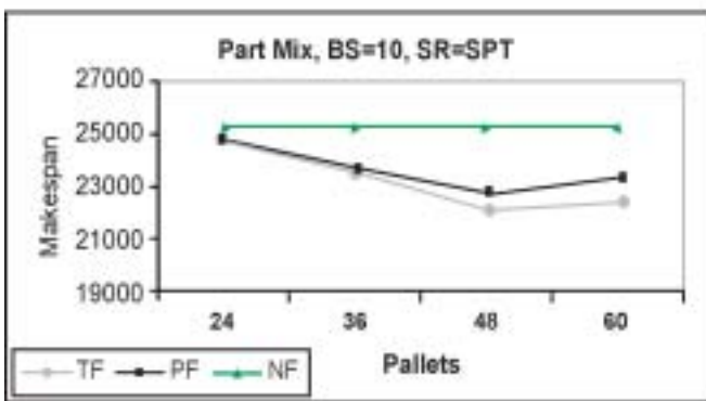
Figure 4: Effect of Part Mix on the System Performance
