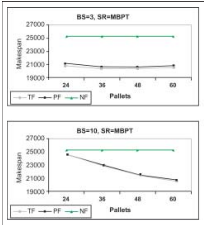
Figure 5: System Performance at ST=0 and SR=MBPT
