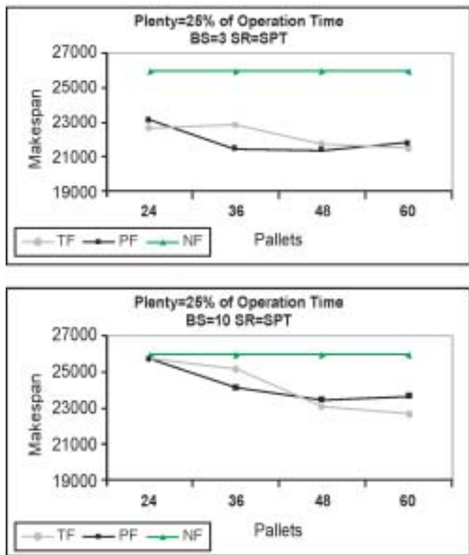
Figure 3: System Performance at Setup=25% of Processing Time
