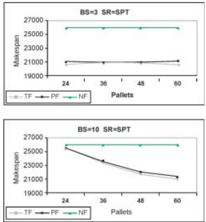
Figure 2: System Performance at ST=0\% and SR=SPT
