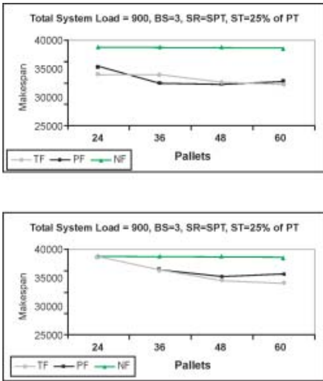
Figure 6: System Performance at System Load=900
